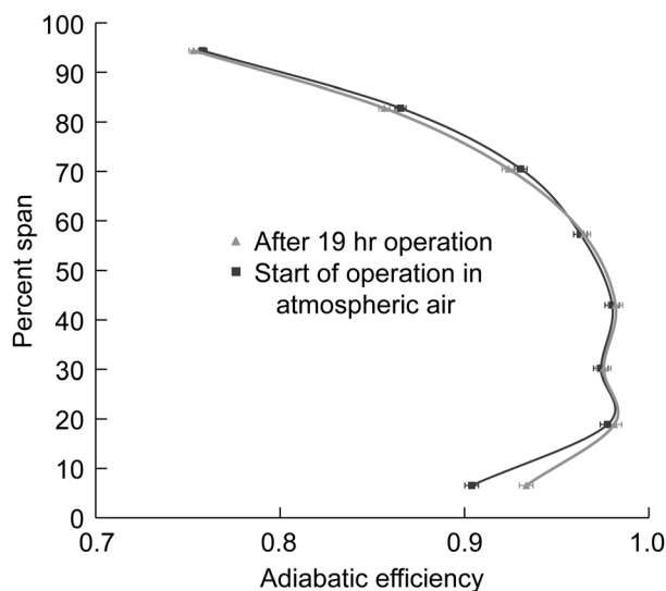
Fig. 12 Spanwise profile of adiabatic efficiency for ultrapolished blade at start of operation in atmospheric air and after 19 h of operation in atmospheric air at 100% speed
